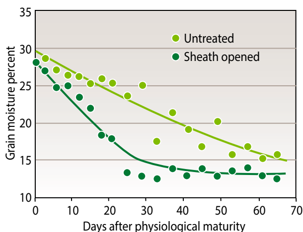
Figure 8. The decrease in moisture content of seed remaining on the plants with time after physiological maturity, where the cob sheath leaves were either opened or untreated. (Data from the Agricultural Research Trust, Harare, Zimbabwe.)
